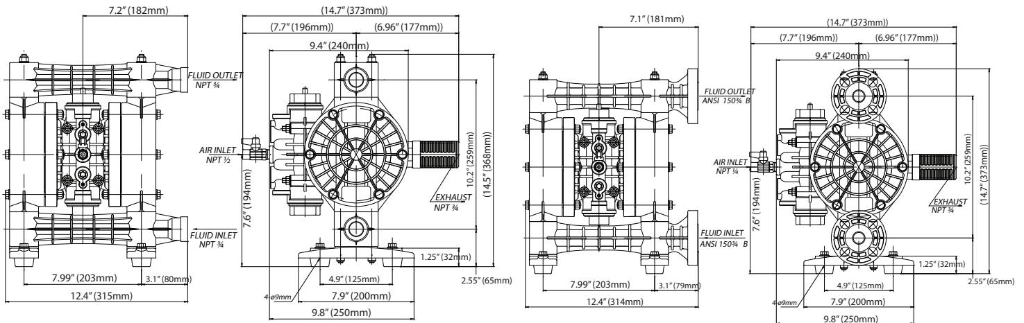
TC-X202P (NPT)
